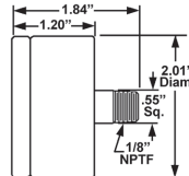
CI-20 - For use with 25 PSI filter by-pass valve
