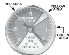
GV-10 - For use with 5 PSI filter by-pass valve
