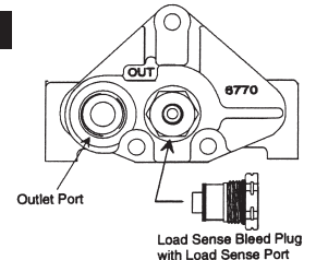
Outlet Cover w/ Bleed Port
