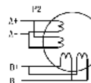
Figure 8: 8-lead motor parallel connections
