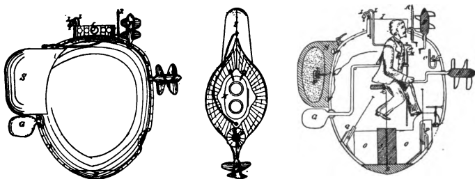
The Best-known Picture of Bushnell's Turtle .
